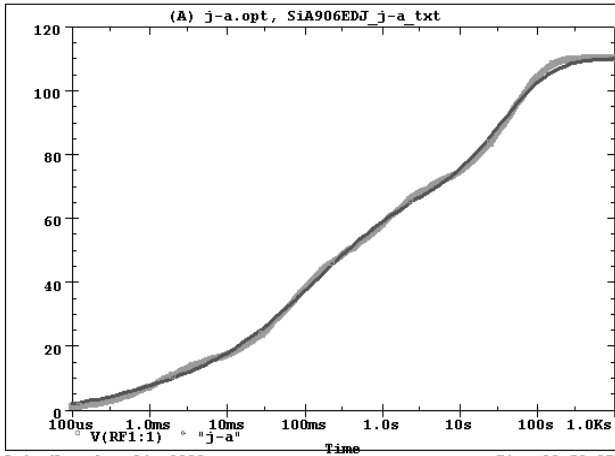
SiA906EDJ Filter j-a Temperature:27.0
