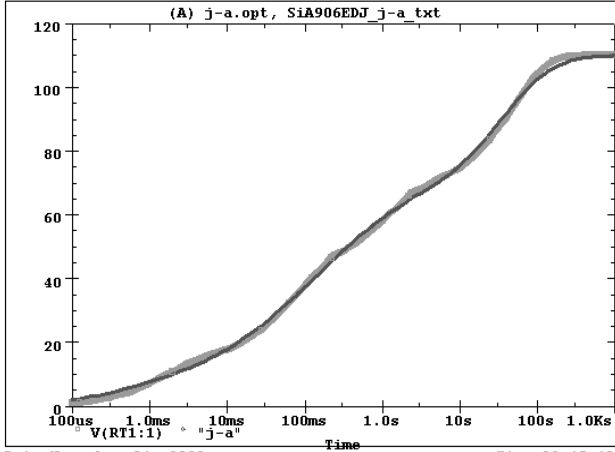
SiA906EDJ Tank j-a Temperature:27.0
