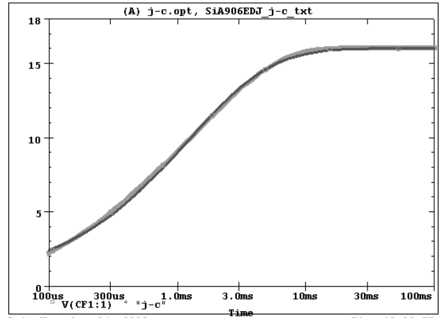
SiA906EDJ Filter j-c Temperature:27.0
