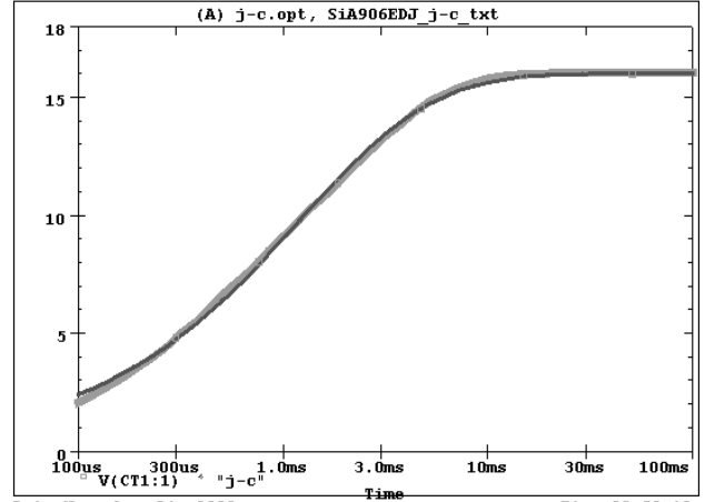
SiA906EDJ Tank j-c Temperature:27.0
